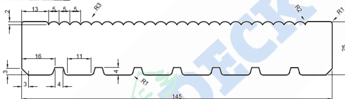
BANGKIRAI 25 x 145 mm – detail profilu
