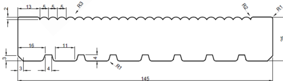
GARAPA 25 x 145 mm - detail profilu
