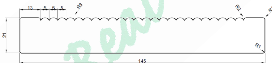
GARAPA 21 x 145 mm - detail profilu
